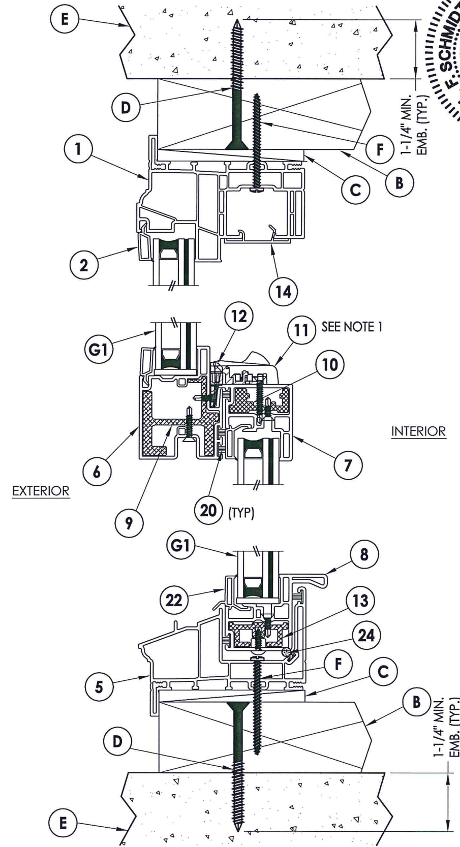
3 VERTICAL CROSS SECTION 2 2X Buck Masonry Construction
