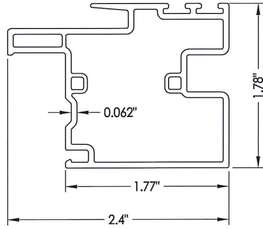
6 MEETING RAIL
