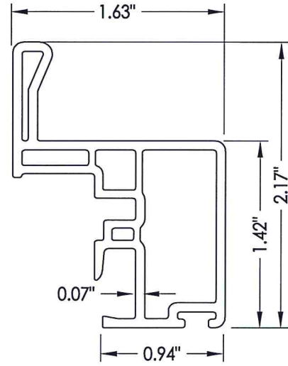
8 BOTTOM RAIL
